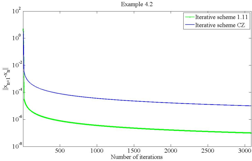
FIGURE 2. Graph showing the convergence of iterative schemes
