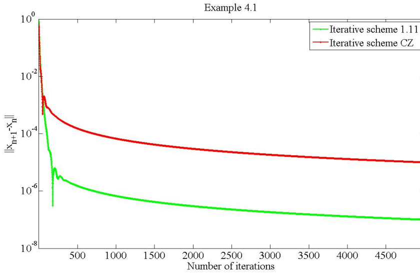
FIGURE 1. Graph showing the convergence of iterative schemes
