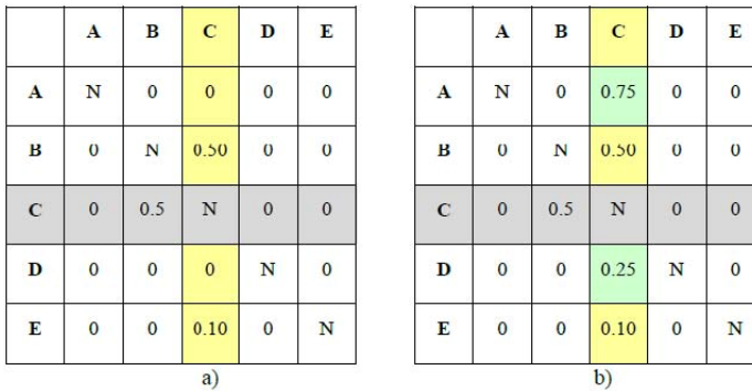
FIGURE 5. a) Step 1: the ant is in C, line C is locked (Grey background). b) Step 2, case 3: the ant ignores the human and computes the probabilities for going to A or D (green cells).
